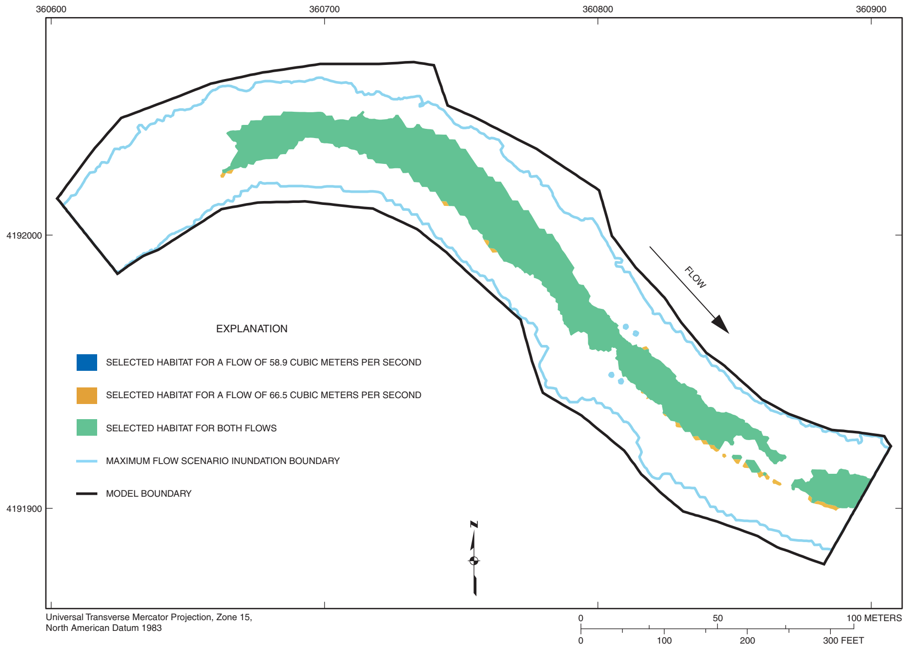
Figure 1-22. Selected habitat area distribution for habitat category 7 (paddlefish) at flows of 58.9 and 66.5 cubic meters per second at Marmaton River site M1.
